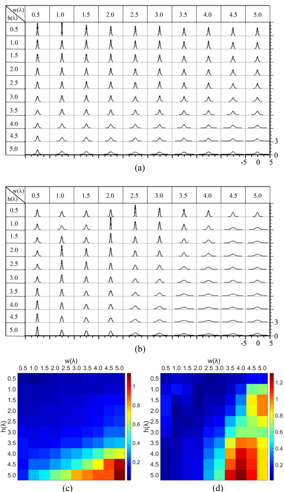
Fig. 1. PDFs and the variances of the real part of one complex rectangular electric field component in perforated enclosures (The first enclosure dimensions are 7.5\lambda \times 7.5\lambda \times 7.5\lambda and the second enclosure dimensions are 10.0\lambda \times 10.0\lambda \times 10.0\lambda ) versus different aperture sizes w(\lambda) and h(\lambda) . (a) PDFs for first enclosure. (b) PDFs for second enclosure. (c) Color image of variances for first enclosure. (d) Color image of variances for second enclosure. Pictures (a) and (b) are extracted from [17].
